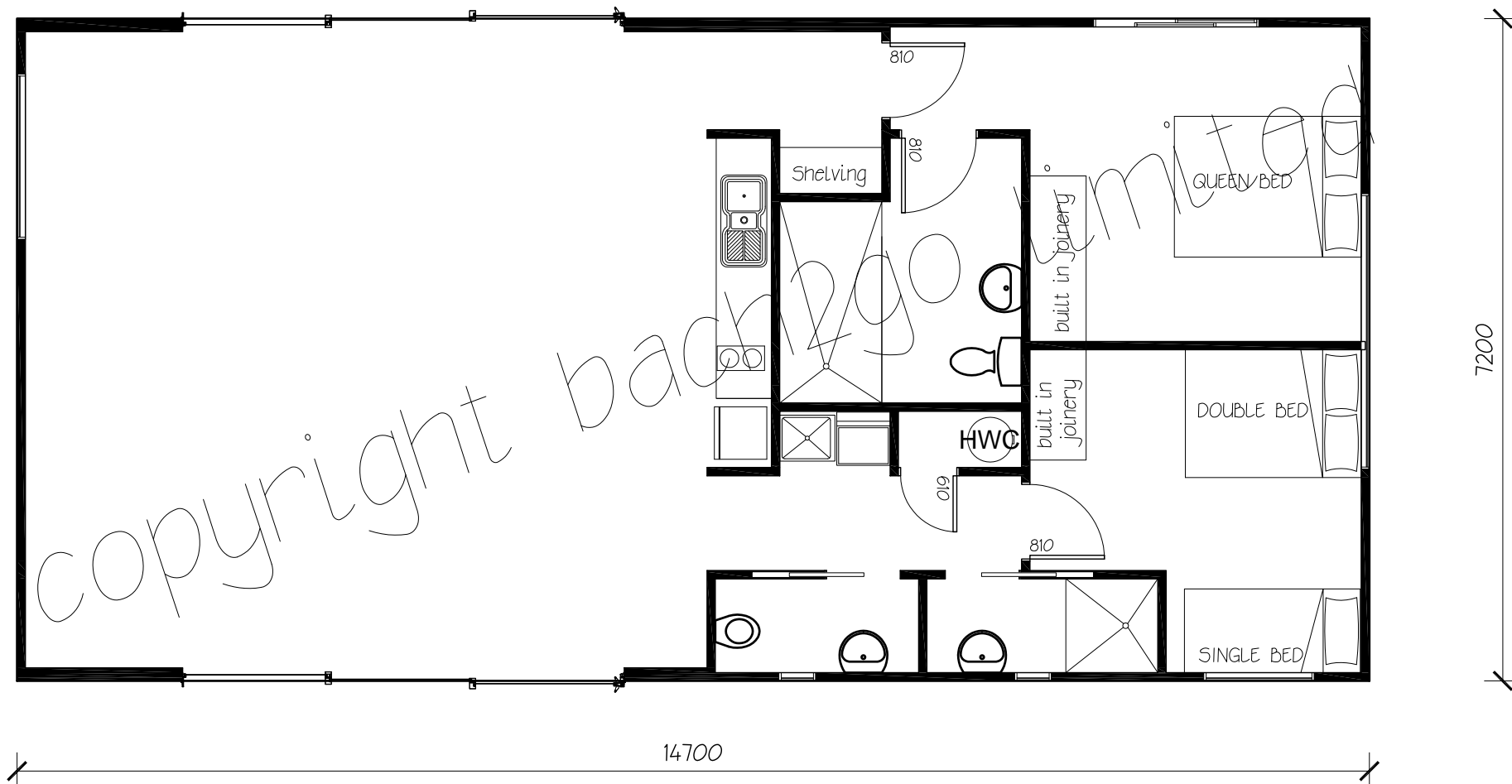
Floor Plan floor area 106m2
